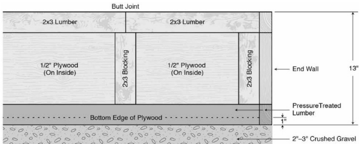
Trough side wall construction.
