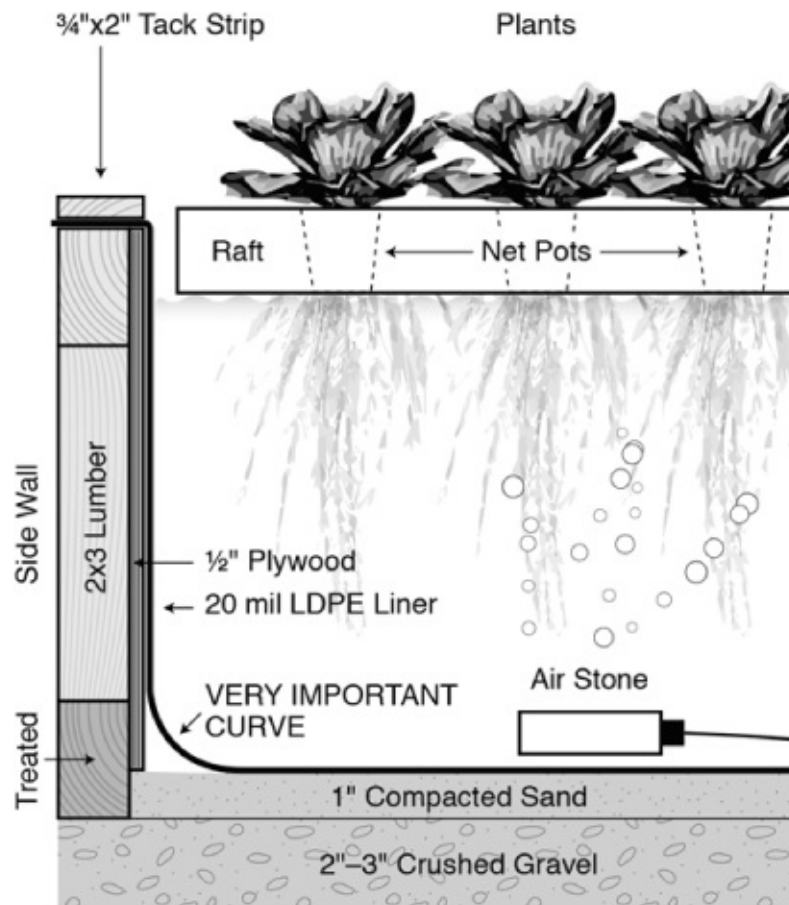
Trough construction as seen from endwall.
