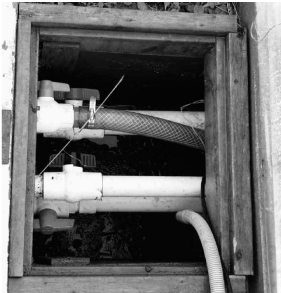
Heat pump and cistern valve service box.
