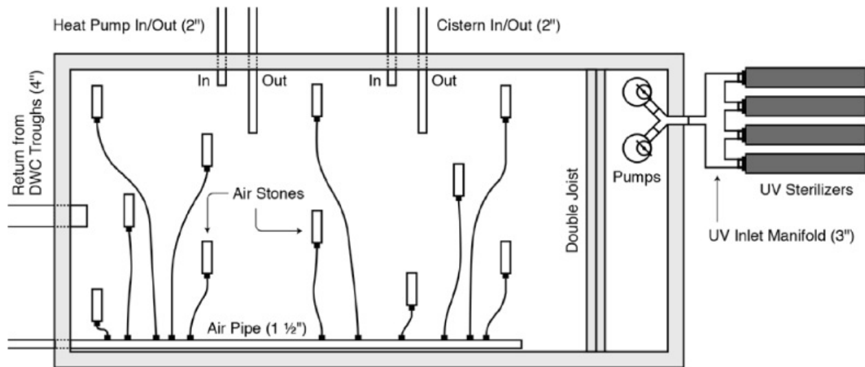
Sump. Top view with cover removed.
